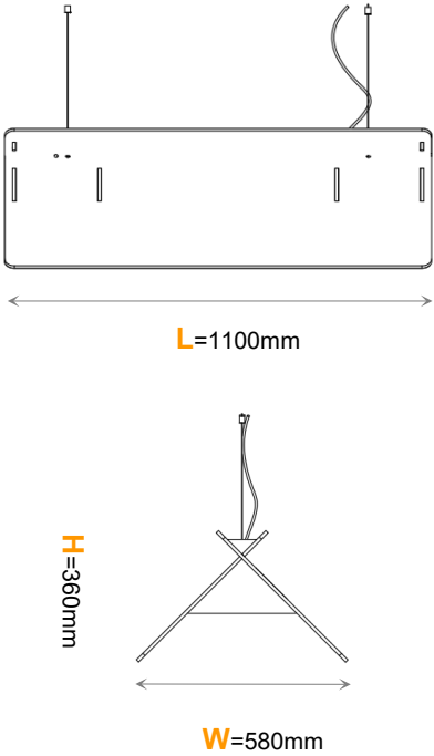
Product Dimensions
